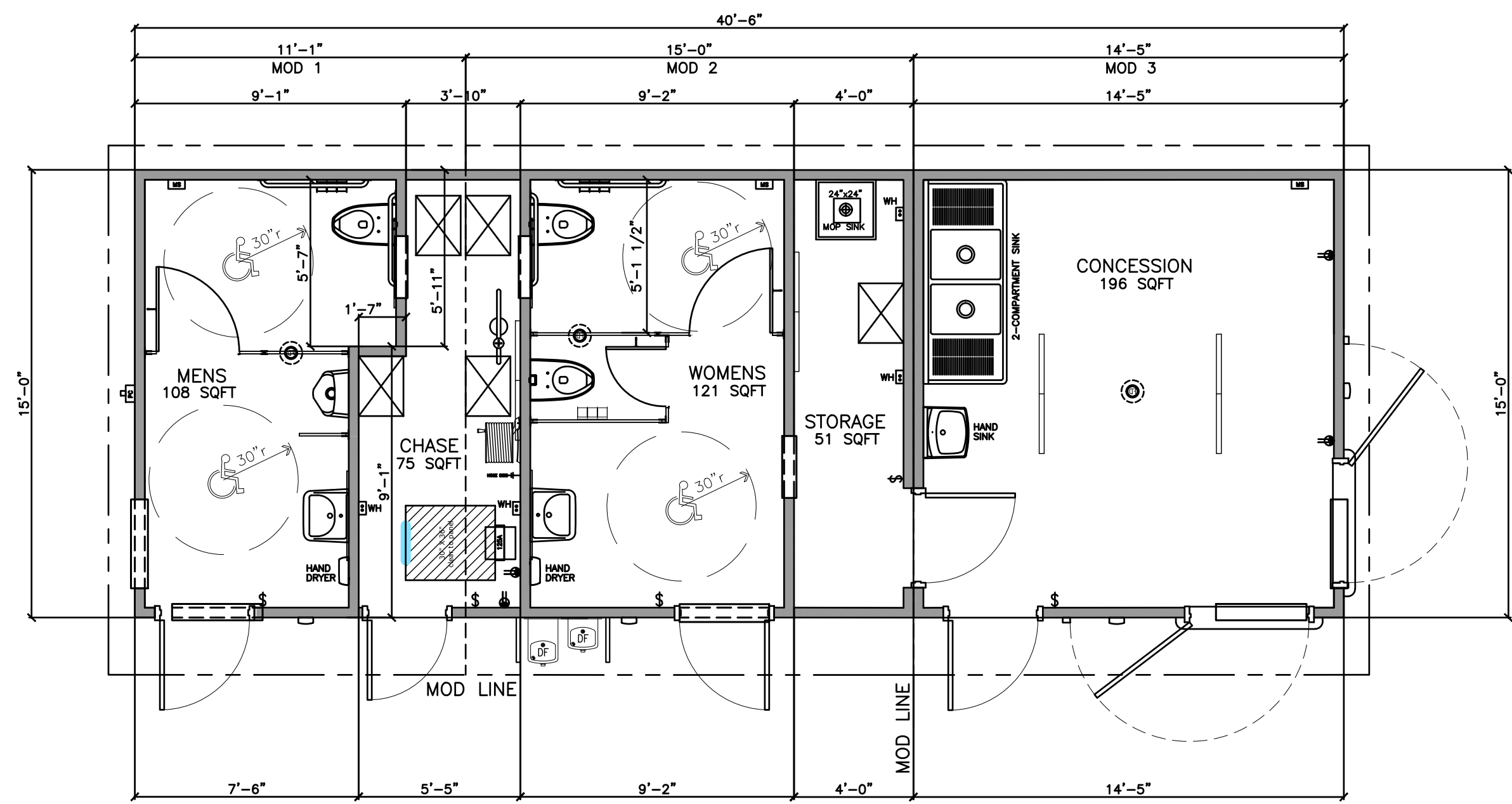
FLOOR PLAN 608 SQFT MIXED OCCUPANCY B/U
