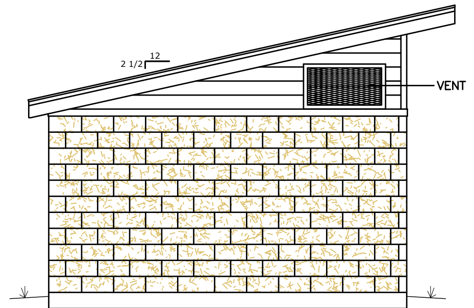
LEFT ELEVATION
